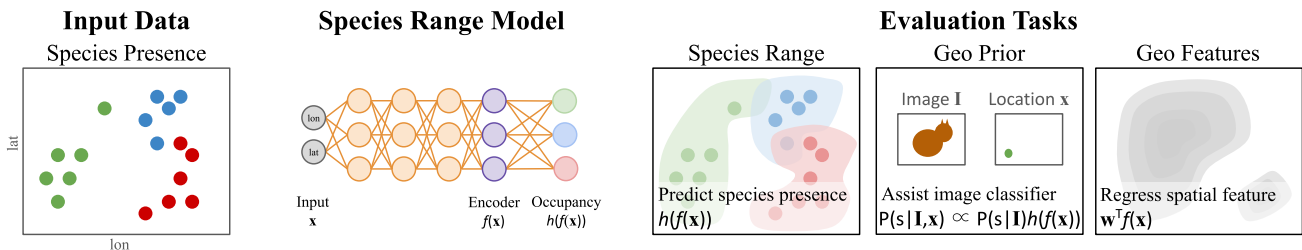
Figure 1. We show that sparse species observation data can be used to train Spatial Implicit Neural Representations (SINRs) which are transferable to other geospatial tasks. (Left) Here we show sparse, presence-only, spatial observations for three toy species (red, green, and blue). (Middle) The species observations are used to train a neural network that consists of a spatial feature encoder and per-species presence predictors. (Right) We evaluate on three diverse tasks: (i) estimating species ranges, (ii) assisting image classifiers using geographical range priors, and (iii) regressing geospatial features via our learned SINR.
