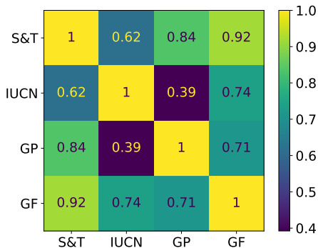
Figure 6. Performance correlations across our four tasks: S&T , IUCN , Geo Prior (GP), and Geo Feature (GF). Values are Pearson product-moment correlation coefficients. The correlations are computed across 12 SINR models: \mathcal{L}_{AN-SSDL} , \mathcal{L}_{AN-SLDS} , and \mathcal{L}_{AN-full} for 10, 100, 1000, and All training examples per class. All models use coordinates as input.
