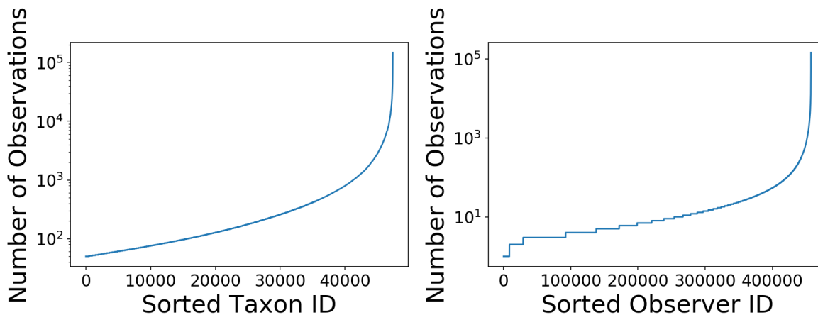
Figure A5. Summary statistics for our training observations data from iNaturalist. (Left) Distribution of observations over species. (Right) Distribution of observations over users (i.e. observers).
