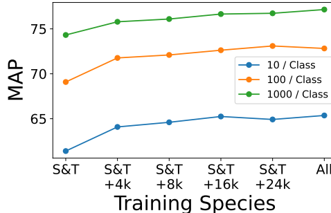
Figure 5. S&T task performance with \mathcal{L}_{AN-full} as a function of the number of training examples per class (i.e. species) and number of classes. The horizontal axis gives the set of species used for training. “S&T” indicates that we only train on the 535 species in the S&T task. For “S&T + X” we add in X species chosen uniformly at random. For “All” we train on all 47k species. Note that the “10 / Class” point for “S&T” is trained with a higher learning rate than usual ( 5e-3 instead of 5e-4 ) due to the small number of training examples per epoch. The values for “All” are also present in Table 1. All models use coordinates as input.
