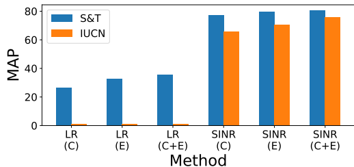
Figure 4. Results for the S&T and IUCN tasks. All models are trained with 1000 examples per class using the \mathcal{L}_{AN-full} loss. We compare logistic regression (“LR”) models against SINR models, using either coordinates (C), environmental covariates (E), or both (C+E) as inputs. These values can also be found in Table 1.
