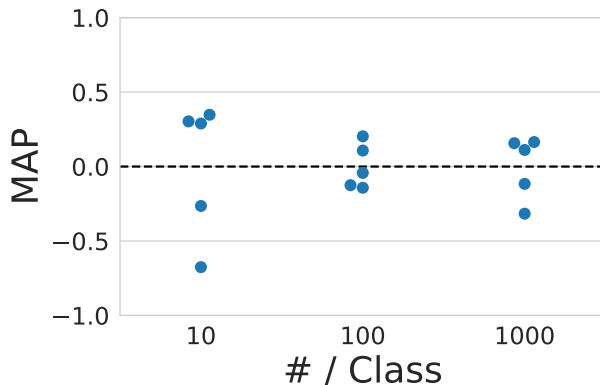
Figure A1. S&T results for SINRs trained with the \mathcal{L}_{\text{AN-full}} loss and varying amounts of training data. For each training data level, we show the mean-subtracted performance for 5 independent training runs. For this figure, the training examples selected for each class are re-sampled for each run. Thus, the randomness we see in this figure combines the randomness due to retraining and the randomness due to training data selection. Deviation from the mean is typically less the 0.5 MAP, and is always less than 1.0 MAP. All models use coordinates as input.
