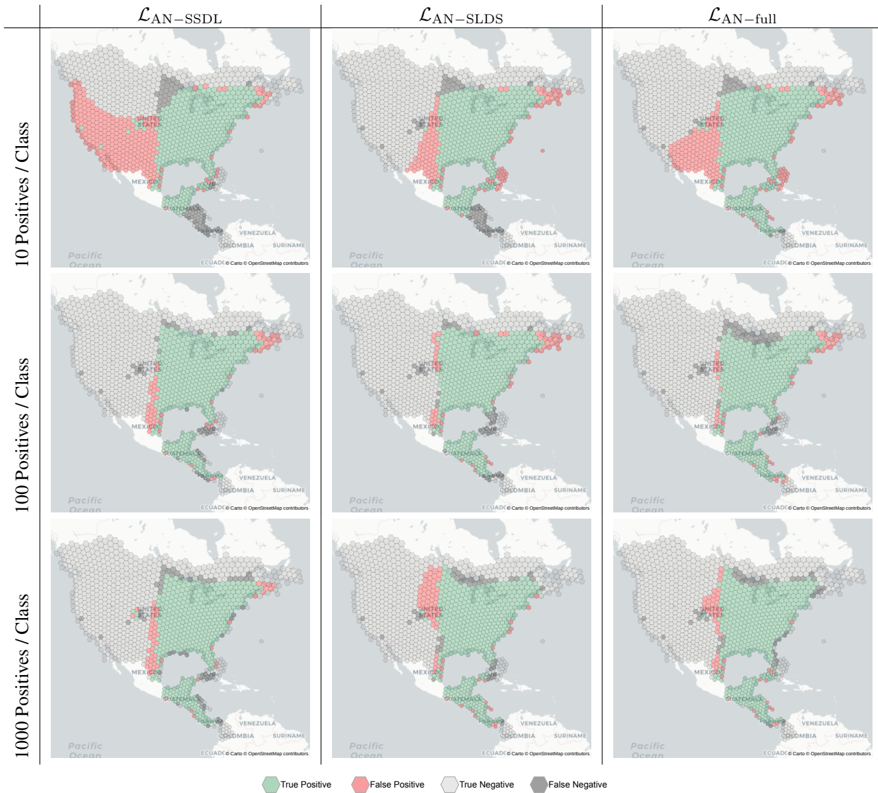
Figure 7. Visualization of SINR predictions for Wood Thrush when varying the amount of training data (rows) for different loss functions (columns). Model predictions are generated at the centroid of the rendered hexagons for a coarse H3 grid (resolution three), signifying locations where we can evaluate the model outputs for the S&T task. We convert the predictions to binary values using the threshold that maximizes the F1 score on the S&T data. This is done for each configuration independently. In practice this threshold would be chosen by a practitioner to meet particular project requirements. A model that matches the S&T task exactly would show only green and light grey hexagons. All models improve their range maps when given access to more data, as expected. \mathcal{L}_{AN-SSDL} overestimates the western range extent and misses the southern extent with few examples, but refines these extents with additional data. \mathcal{L}_{AN-full} starts off with most of the range covered (few “False Negative” hexagons) and proceeds to tighten the boundaries with more data. The range predicted by \mathcal{L}_{AN-SLDS} is somewhere in between. All models use coordinates as input.
