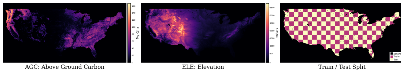
Figure A8. Here we illustrate two of the nine evaluation layers used in the Geo Feature prediction task (left and middle). On the right we indicate which regions contain pixels that are in the train or test split, or simply ignored during evaluation.
