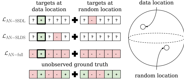
Figure 2. Illustration of the data used by three loss functions from Section 3.2. For each loss, we visualize the targets that the network is trained to predict. Each loss can be broken into two parts: one part that updates the network’s predictions at the location of a training example ( data location ) and one part that updates the network’s predictions at another location chosen randomly ( random location ). Each loss has access to one confirmed positive label (bold boxes). The rest of the labels are unobserved (non-bold boxes), and the losses make different, imperfect, assumptions about those unobserved labels.
