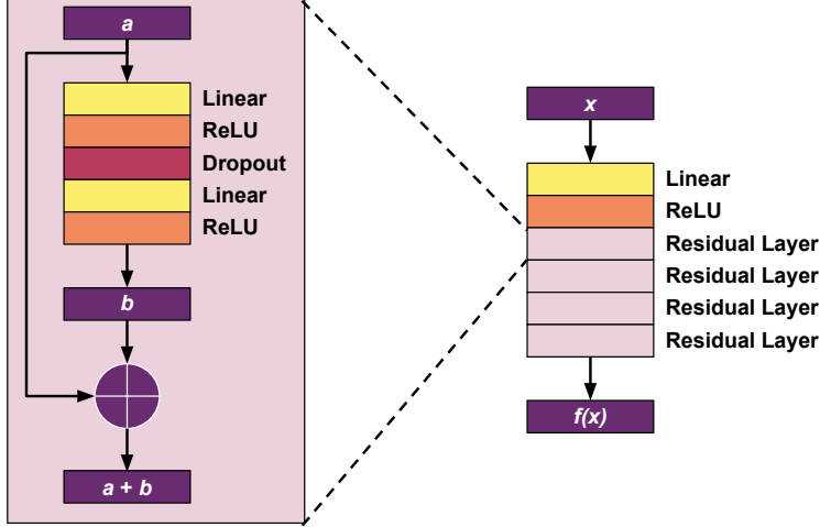
Figure A3. Network diagram for the fully connected network (with residual connections) which we use for our location encoder f_\theta .
